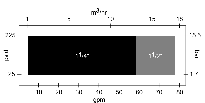
T166 Performance Curve
