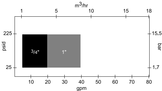
B166 Performance Curve
