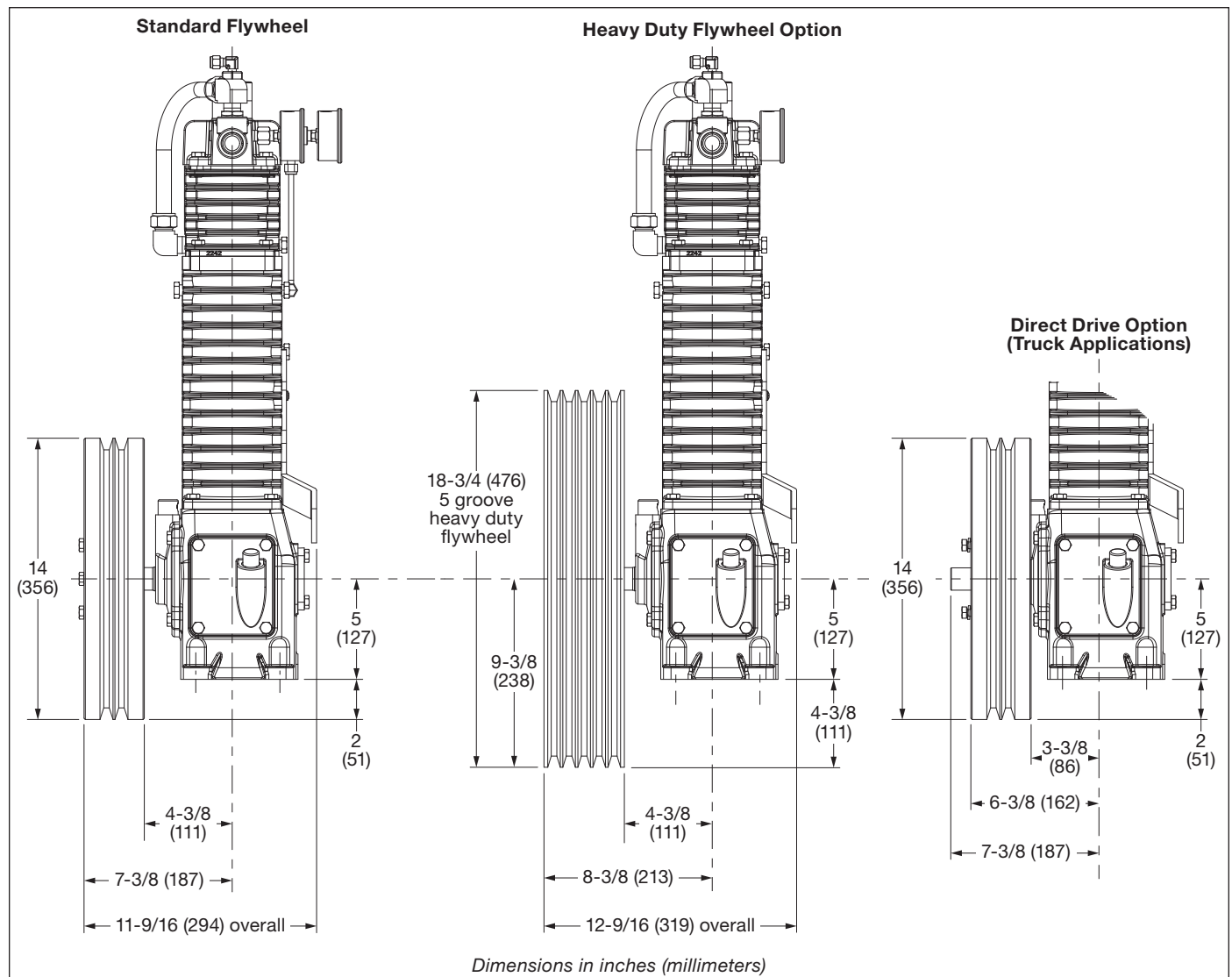
For illustration purposes, a model D91 is shown above but the dimensions apply to all model 91 compressors.
