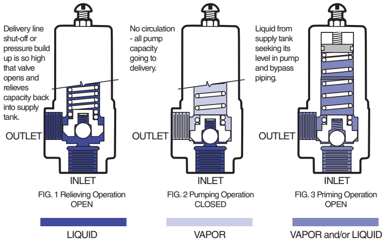
Corken B166 Bypass Valve Functions.
